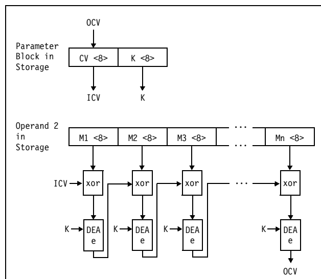
Figure 7-77. KMAC-DEA
