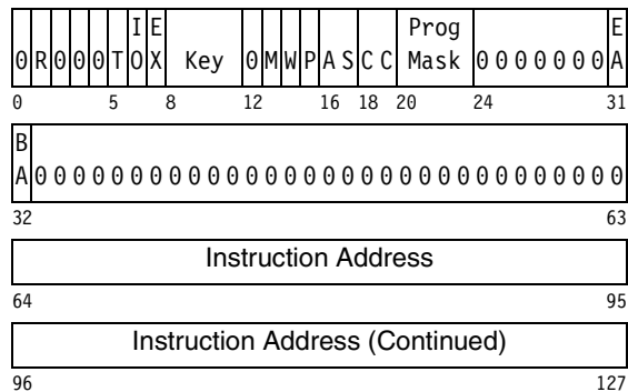
Figure 4-2. PSW Format
