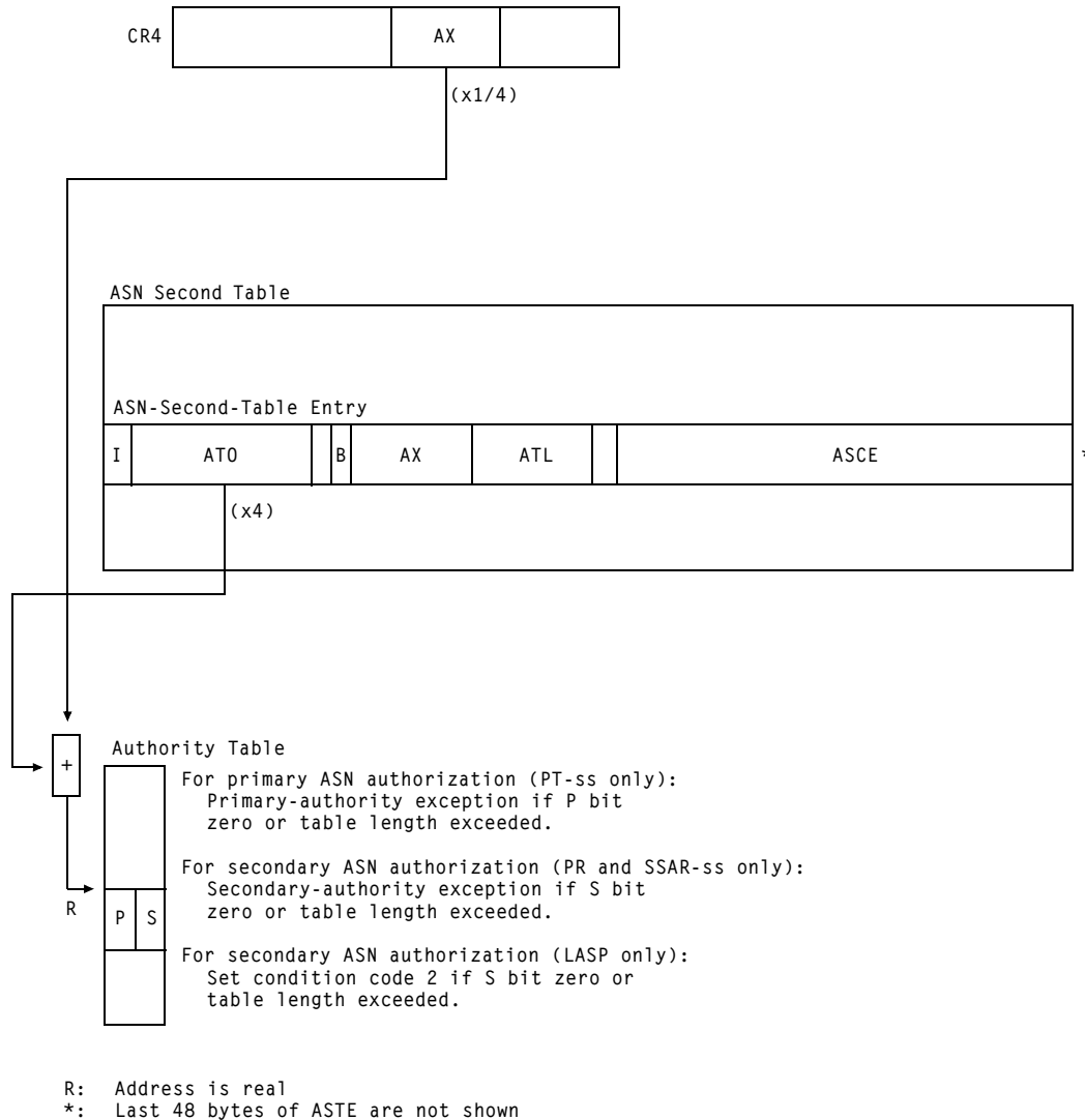
Figure 3-8. ASN Authorization
