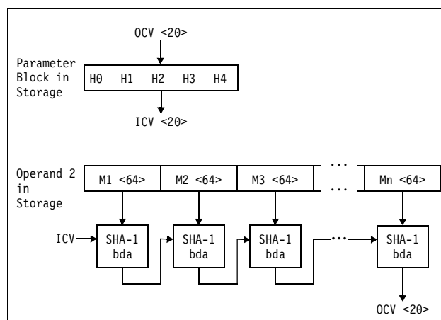
Figure 7-56. KIMD-SHA-1
