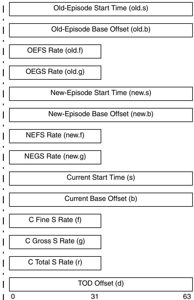
Figure 4-11. TOD-Clock-Steering Registers
