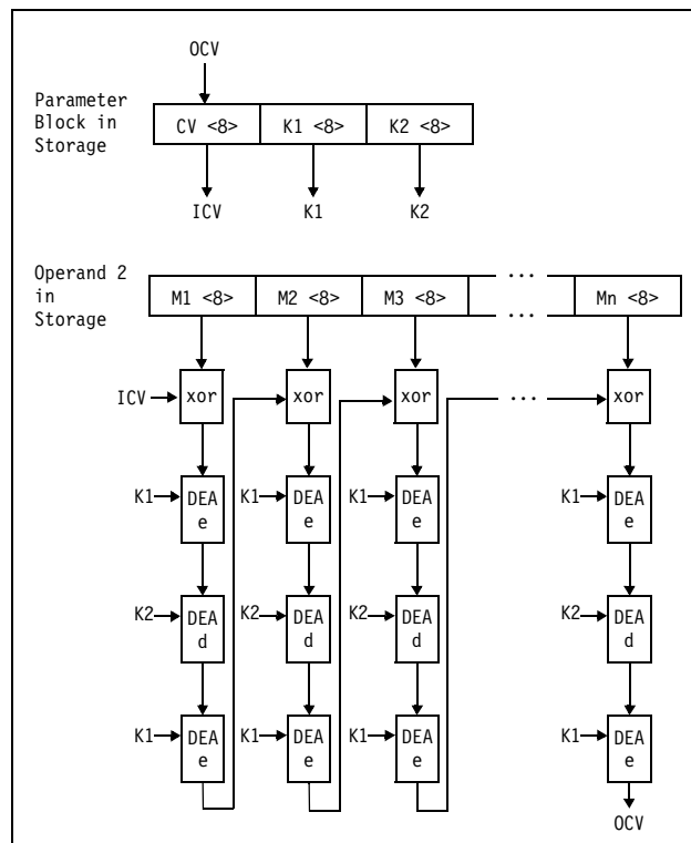
Figure 7-79. KMAC-TDEA-128
