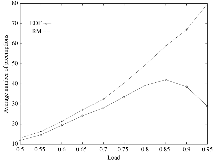
Figure 3. Preemptions introduced by RM and EDF on a set of 10 periodic tasks as a function of the load.
